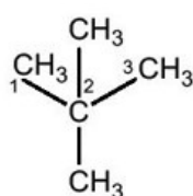
2,2-dimethylpropane (neopentane)
