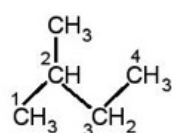
2-methylbutane
