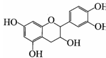
Catechin
